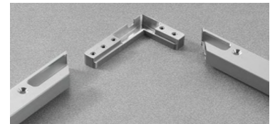
Corner assembly
